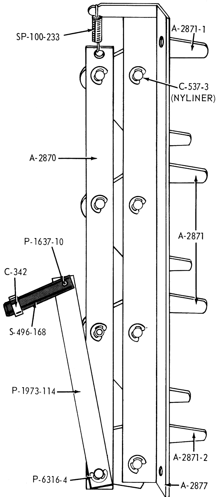
FREE BALL ESCAPE ASSY. AS-2300
