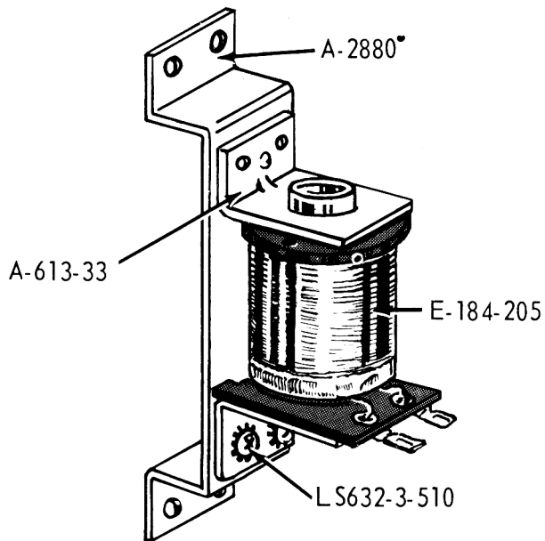
COIL & BRACKET ASSEMBLY AS-2299
