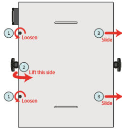
Figure E22. Removing PCB chassis lid.
