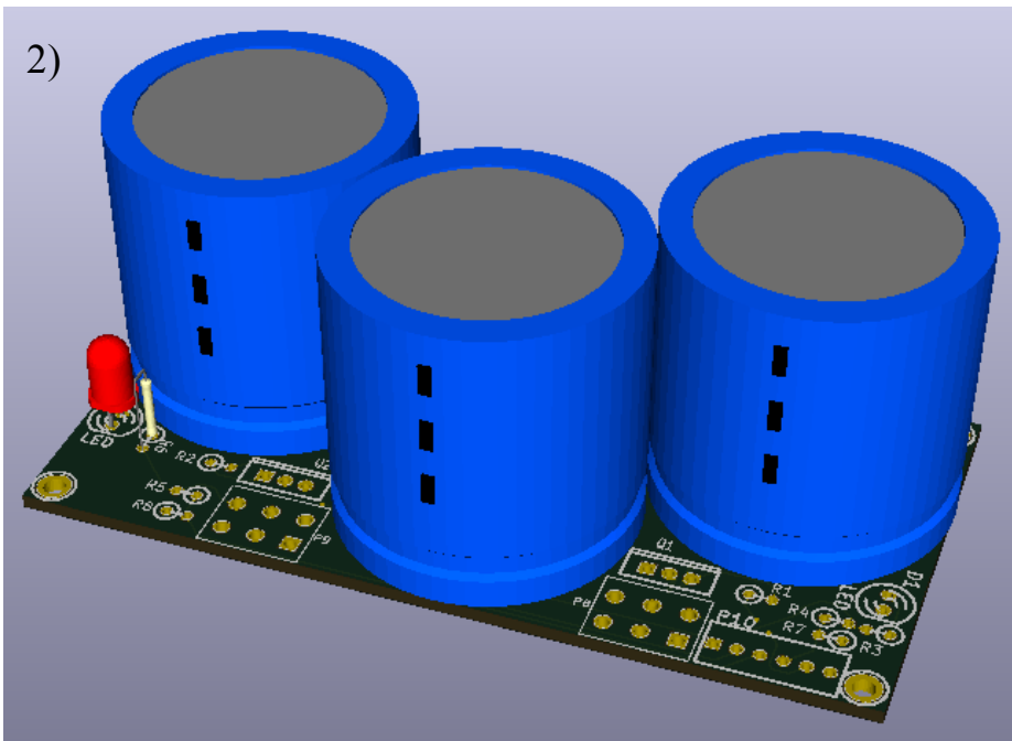
2) LED (D2) and bleeder resistor (R6) installed.
