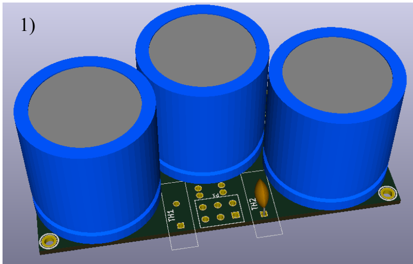
1) Three capacitors (C1, C2, C3) & thermistor (TH2) installed.
